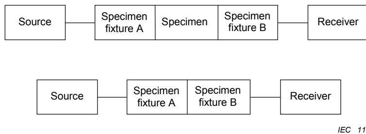
Figure A.1a – Insertion technique
